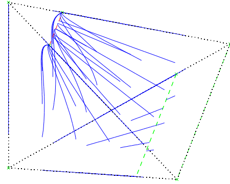
Fig. 3. Stationary points in the simplex. Nash equilibria are represented using a red dashed line, and other stationary points are in dashed green lines. Solid lines show sample trajectories. In particular, the entire facet \{\mu : \mu_1 = \mu_2 = 0\} is stationary.
