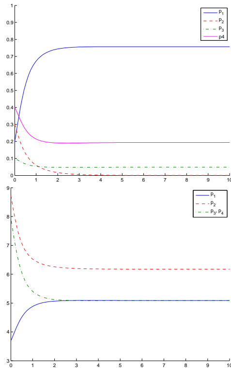
Fig. 1. Trajectory of \mu(t) (top) and evolution of loss functions (bottom). We have convergence to the set of Nash equilibria: on the support of the limit distribution, all bundle losses are equal.
