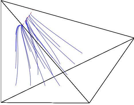
Fig. 2. Trajectory of \mu(t) in the simplex \Delta^{\mathcal{P}} (represented as a tetrahedron). Starting from different initial conditions, we have convergence to different points in \mathcal{N} (represented with a red dashed line).
